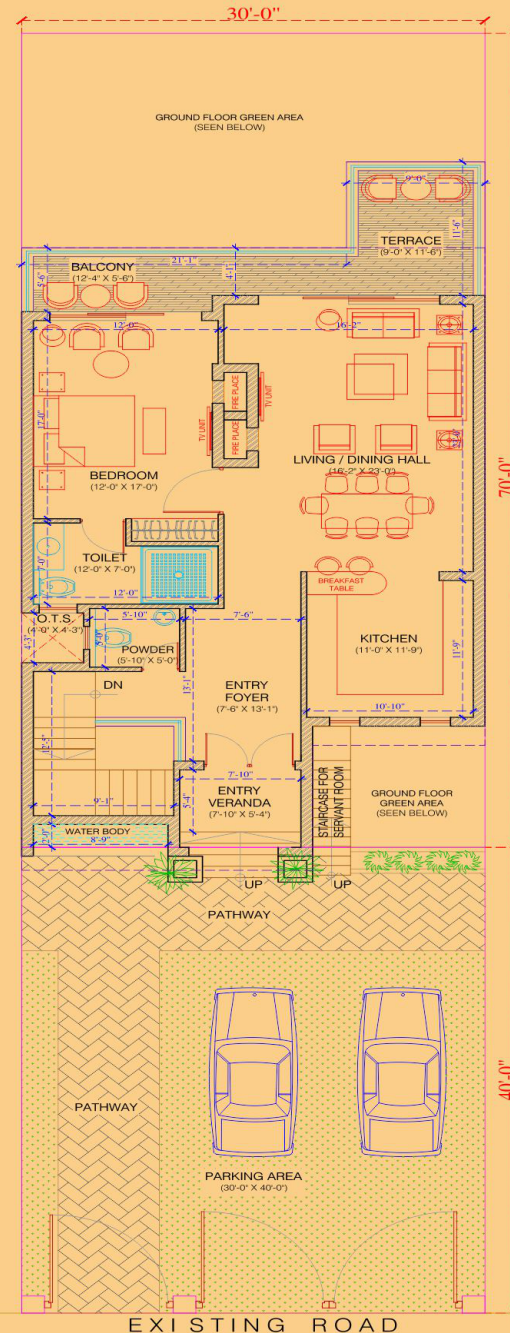
FIRST FLOOR PLAN - R2
