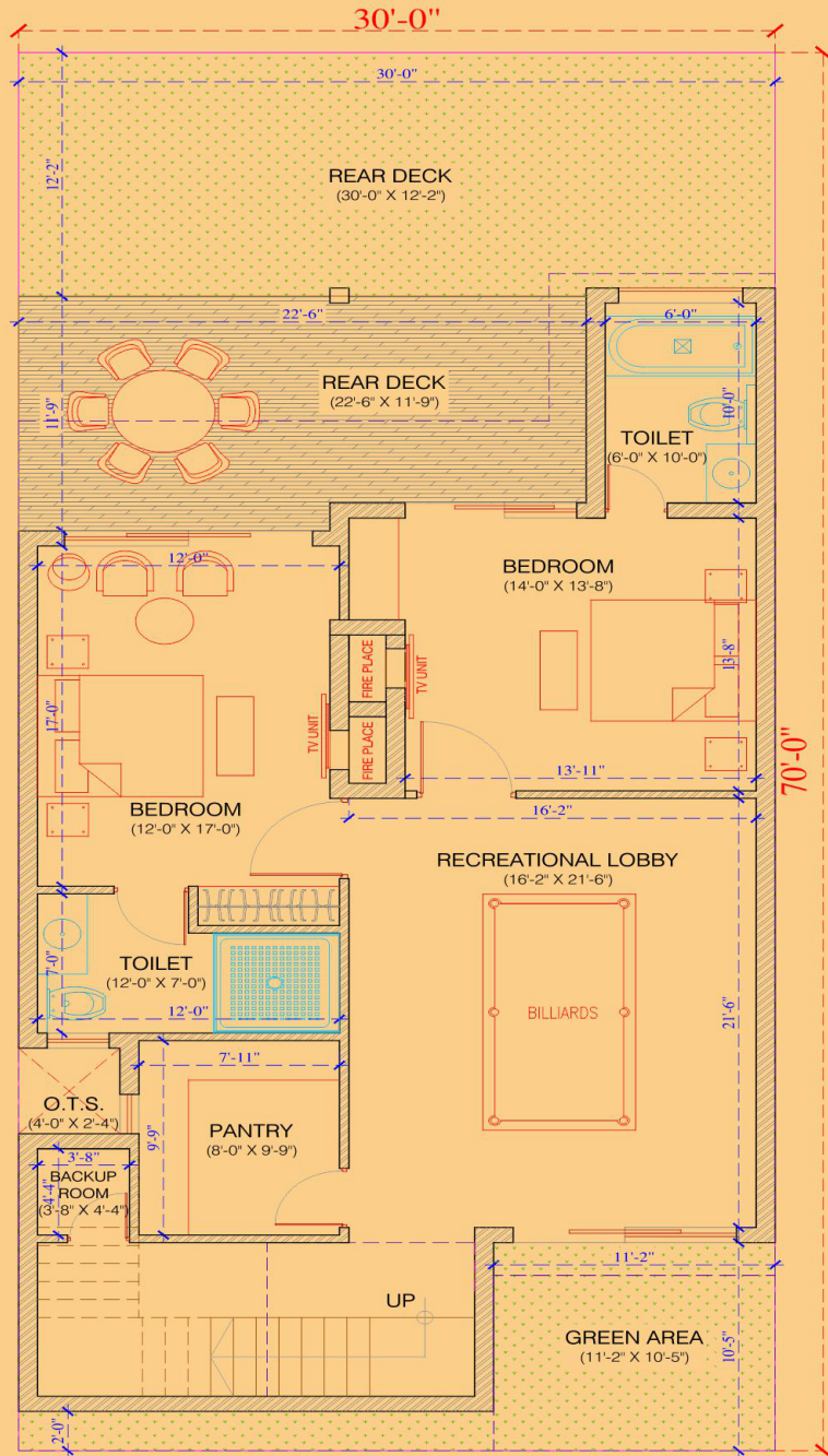
GROUND FLOOR PLAN - R2
